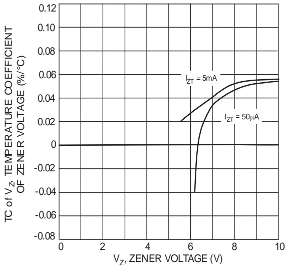
Fig. 12 Typical Temperature Coefficient of Zener Voltage vs. Zener Voltage, DDZ6V2BS-DDZ10CS
