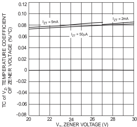
Fig. 14 Typical Temperature Coefficient of Zener Voltage vs. Zener Voltage, DDZ20CS-DDZ30DS
